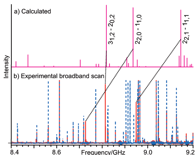
Figure 1. a) Simulated 0.8 GHz section of the rotational spectrum of ML... 14 NH 3 I using the spectroscopic constants reported in Table 1 with T_{\text{rot}} = 1 K. b) 0.8 GHz sections of two broadband chirped-pulse microwave scans using ML + NH 3 + Ne (solid red) and ML + Ne (dashed blue) samples. The scan of NH 3 + Ne is not shown since the transitions observed are very weak in this frequency region.
